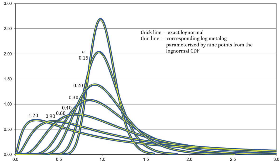
Figure 1: Exact lognormals vs. corresponding metalog distributions.
